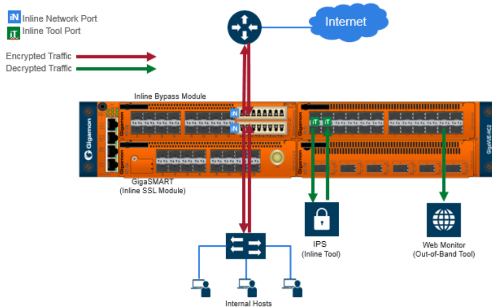
Figure 46 GigaVUE Modules: GigaSMART and Inline Bypass
