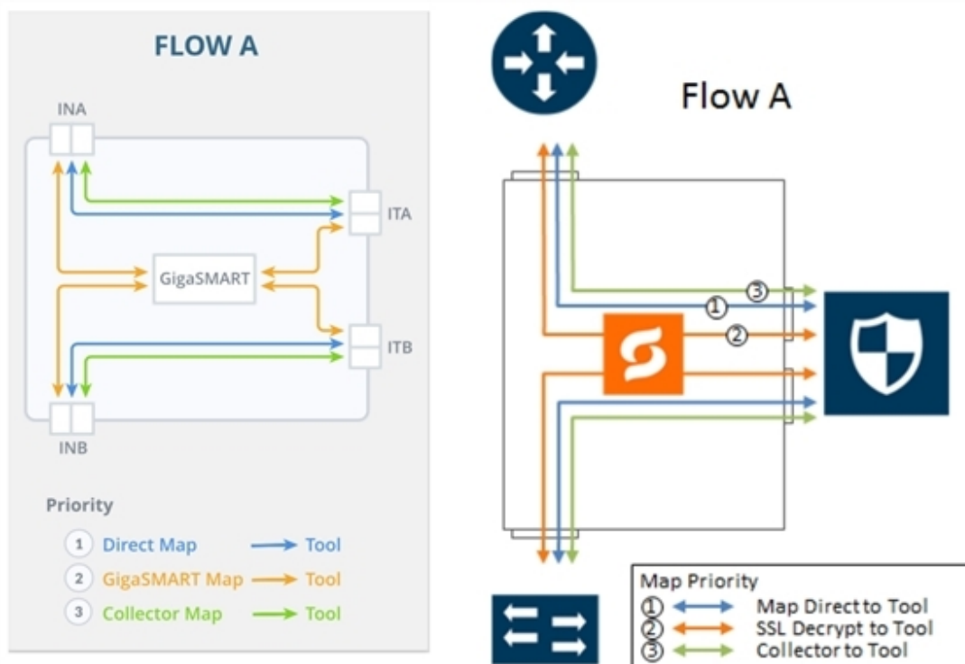
Figure 52 FLOW A Views
