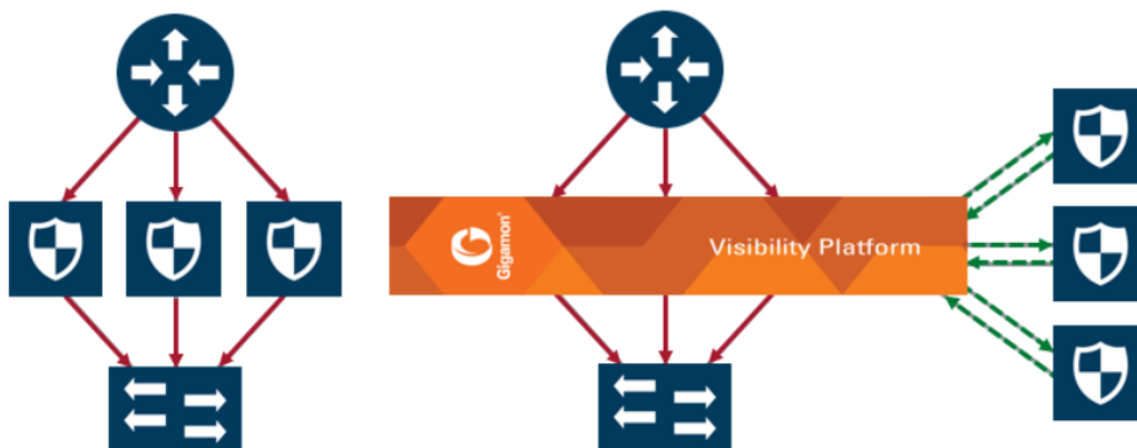
Figure 42 Multiple Inline Tool Arrangement
