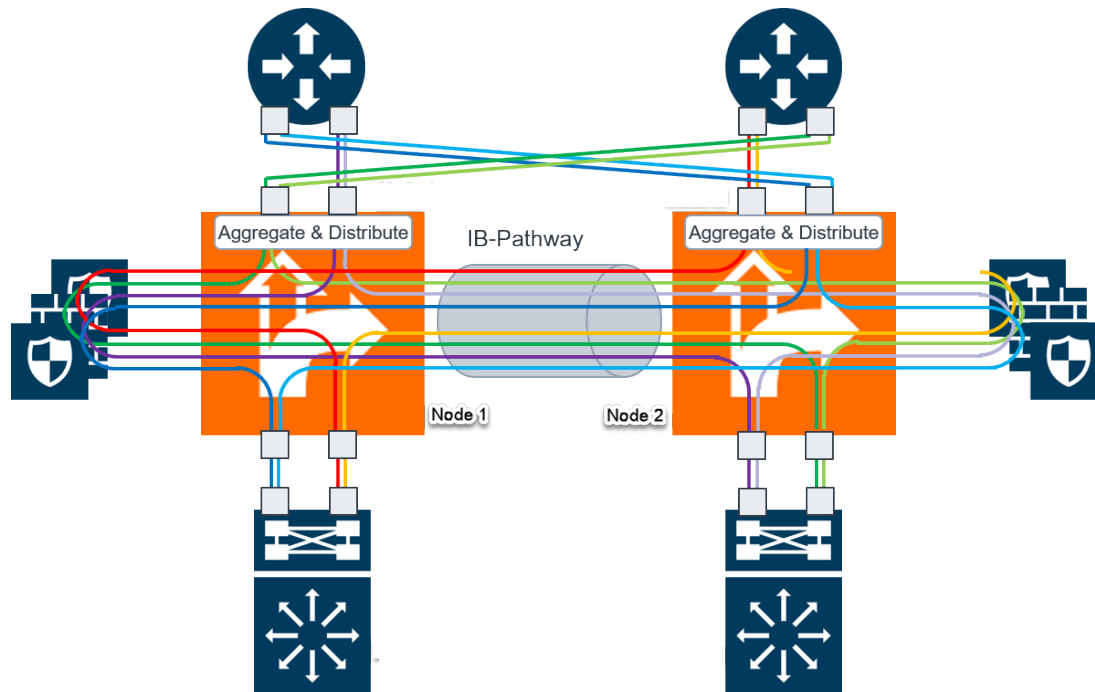
Figure 12 Resilient Inline Arrangement
