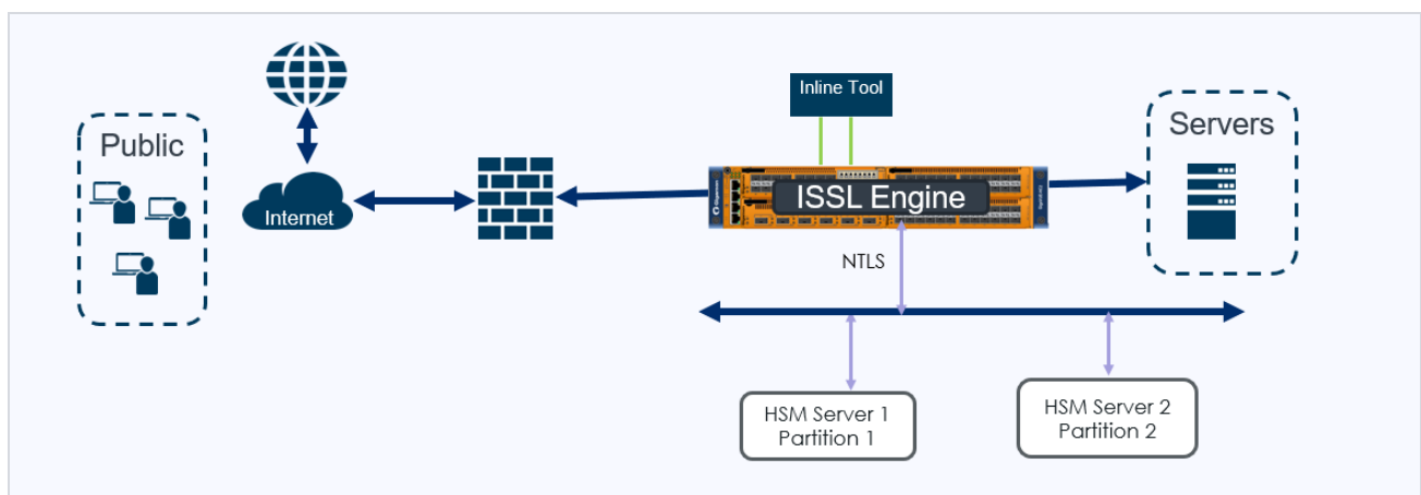
Figure 13 ISSL with Thales Luna - Inbound support
