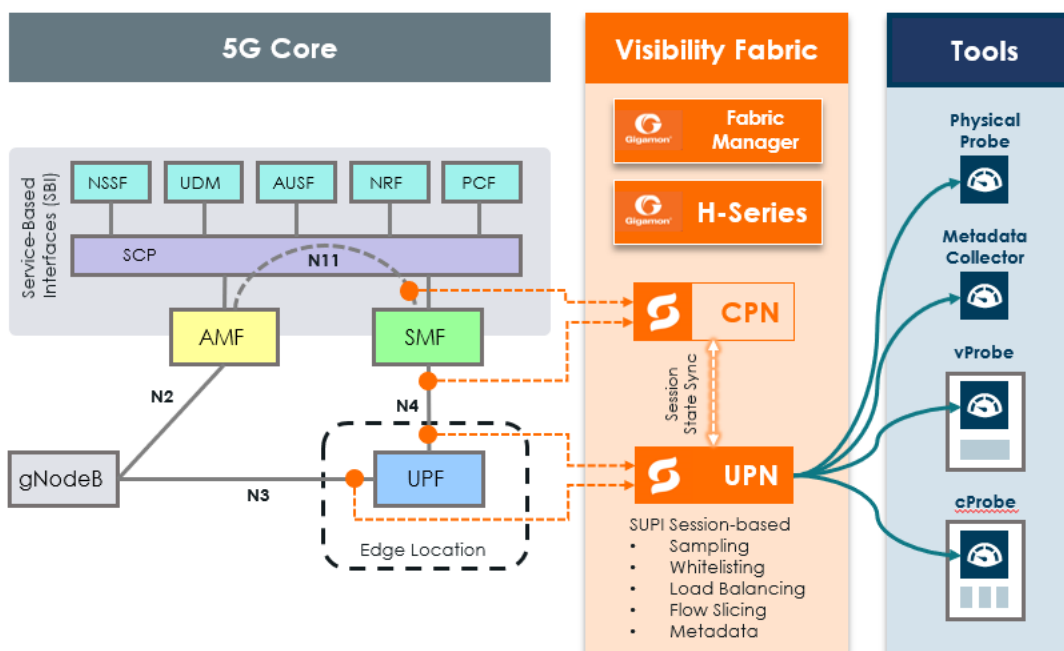
Figure 22 5G Stand Alone Packet Core Network
