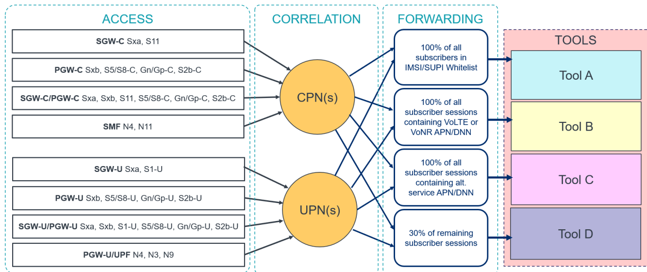
Figure 23 CUPS Traffic Visibility Solution
