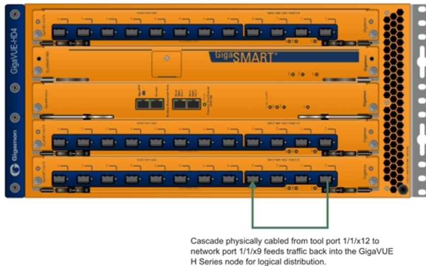
Figure 152 Cascade Physically Cabled from Tool to Network Port
