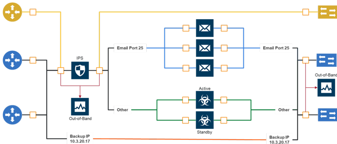
Figure 10 Flexible Inline Arrangements Scenario
