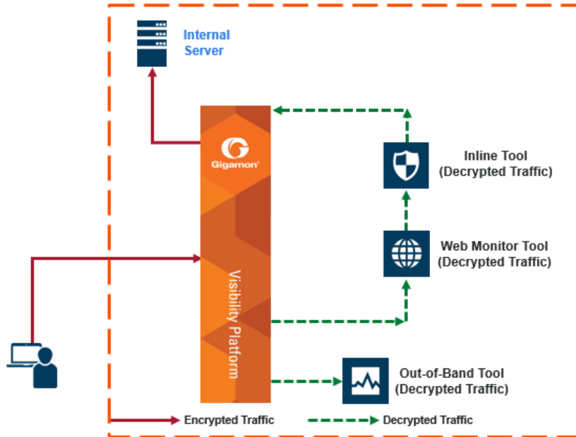
Figure 44 Inbound Deployment of Inline TLS/SSL Decryption
