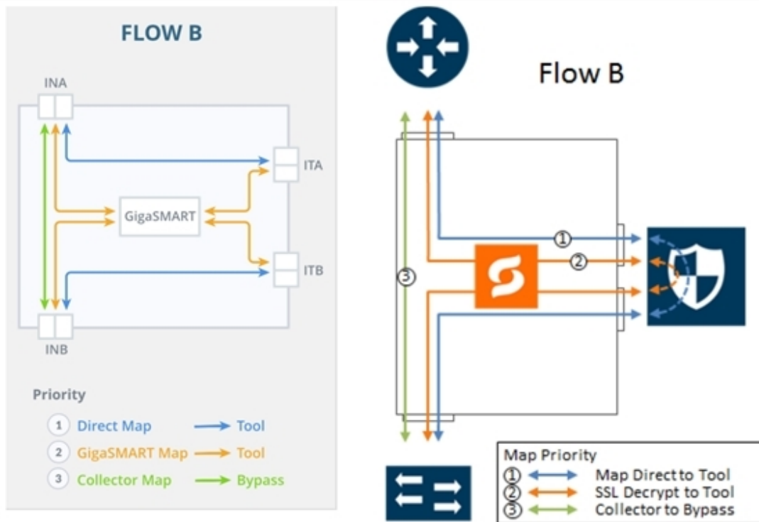
Figure 53 FLOW B Views
