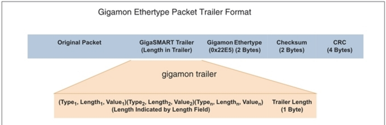
Figure 154 GigaSMART Trailer Format
