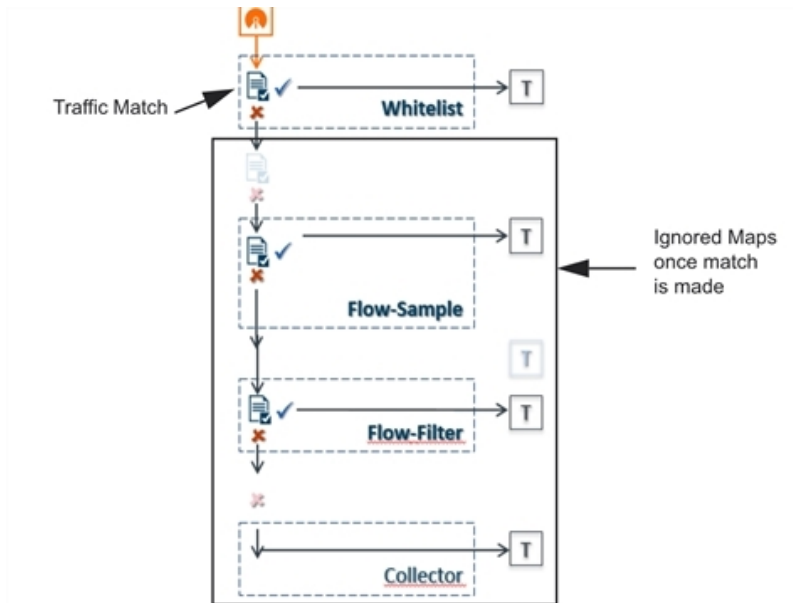
Figure 27 Non-Overlap GTP Mapping Mode
