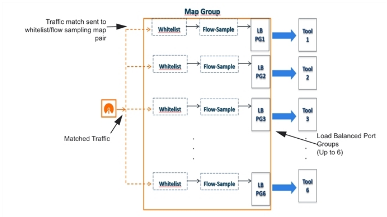
Figure 28 GTP Overlap Flow Sampling Map Groups
