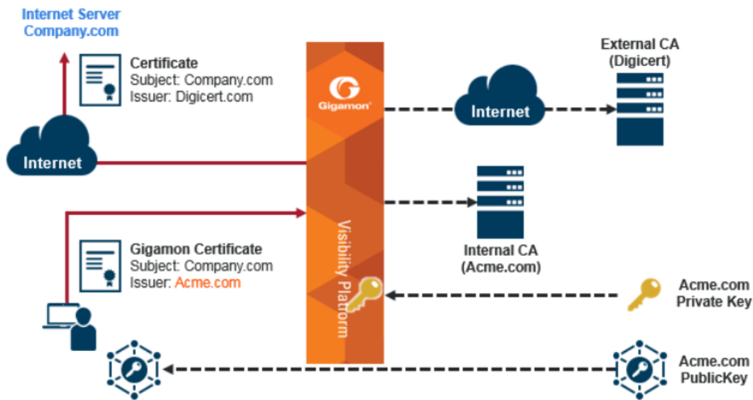
Figure 45 Outbound Deployment of Inline TLS/SSL Decryption
