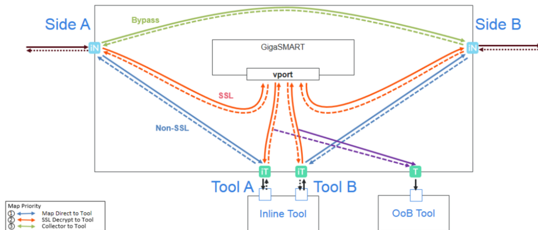
Figure 47 Packet Flow for Inline SSL Decryption
