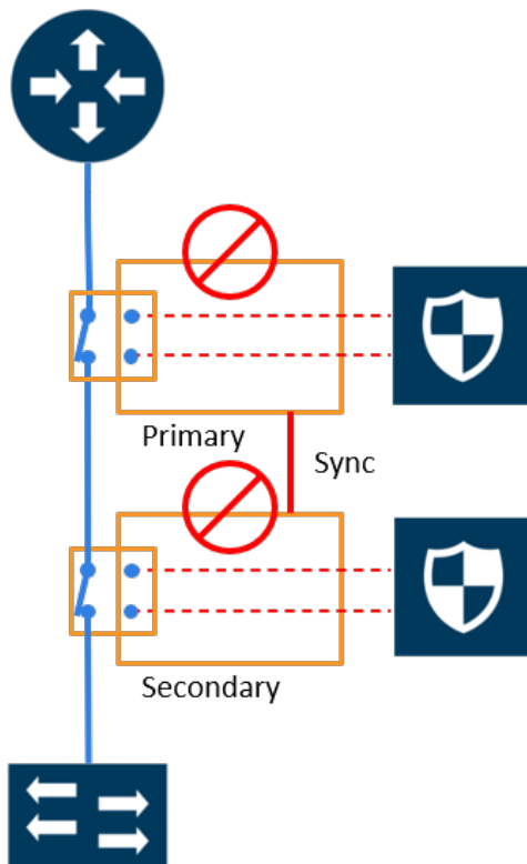
Figure 22 Both Nodes Fail; No Traffic Monitoring
